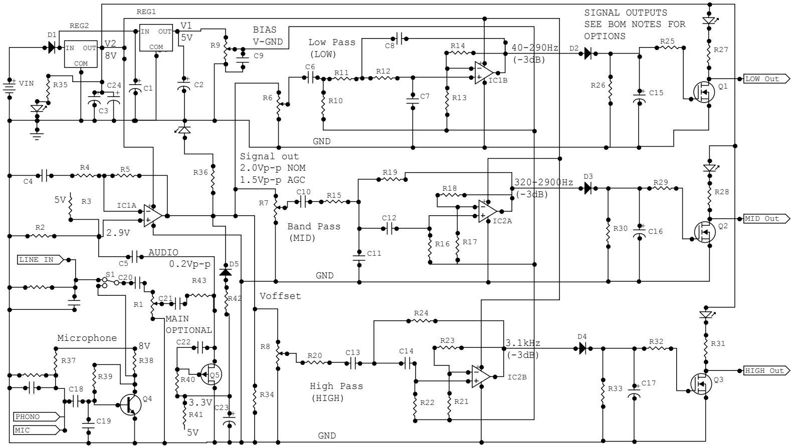
Audio bandpass filter
