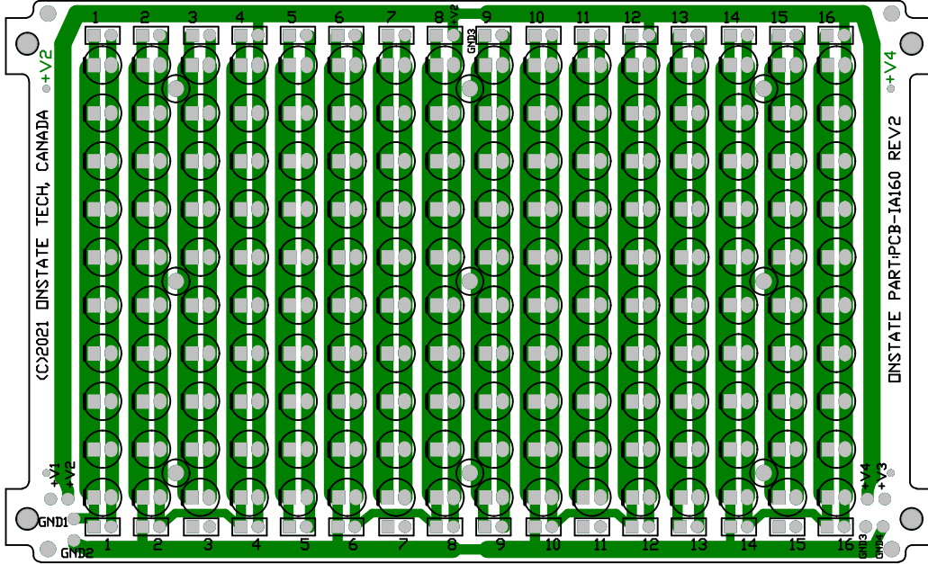
IA160 Top Layer Trace
