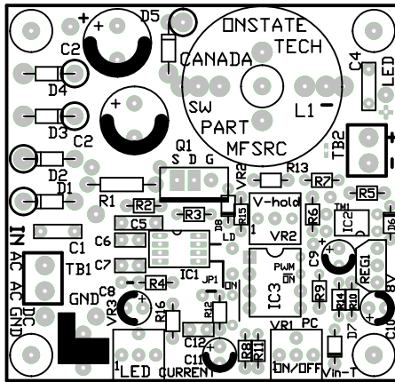
SILKSCREEN LAYER
