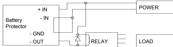
Figure 2. Relay output wiring.
