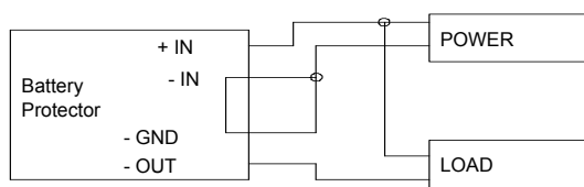
Figure 1. Standard wiring with N-CH MOSFET.
