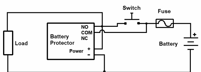
Figure 4. Total shutoff with reset switch.
