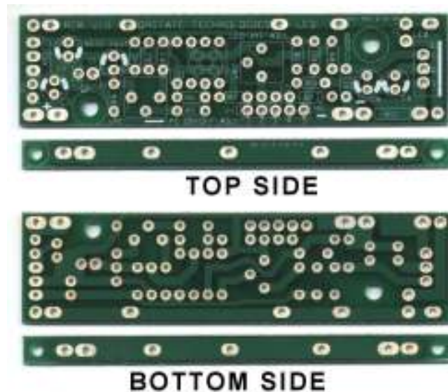
Top and bottom sides of PCR PCB. Detachable bus bar for LED connections.
